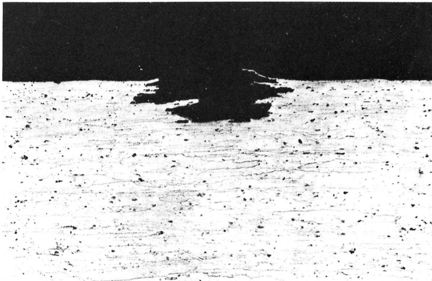
Undermining pitting that may form the surface give the appearance of incipient exfoliation (Keller's Etch; 100x).
